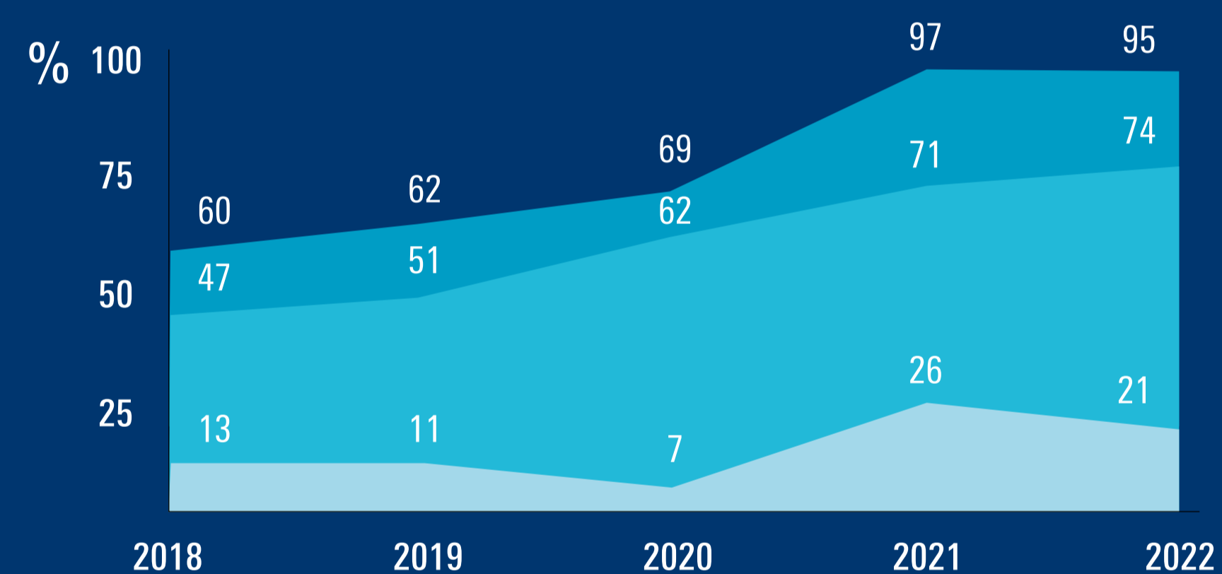
PERCENTAGE OF UT OA PUBLICATIONS IN REFEREED JOURNALS
